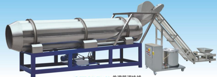
GTW-D-II 单滚筒调味线 Flavoring Line
